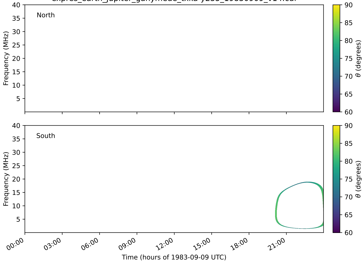
expres_earth_jupiter_ganymede_txka-y235_19830909_v14.cdf
