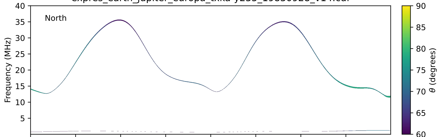
expres_earth_jupiter_europa_txka-y235_19830928_v14.cdf
