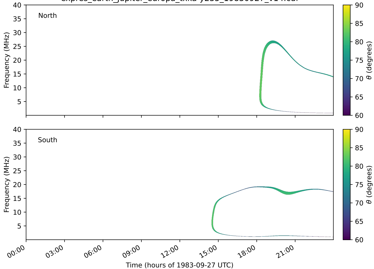
expres_earth_jupiter_europa_txka-y235_19830927_v14.cdf
