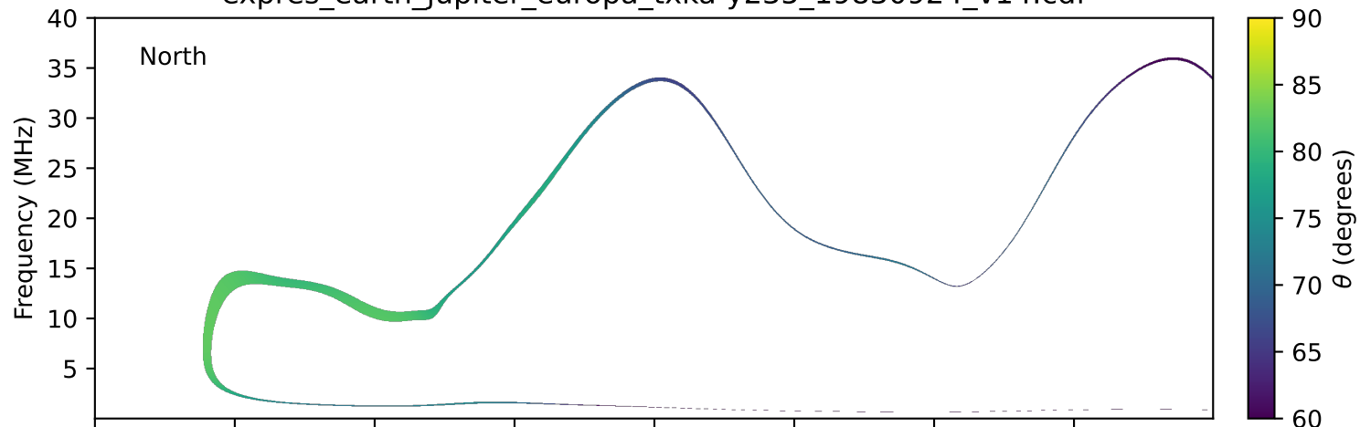
expres_earth_jupiter_europa_txka-y235_19830924_v14.cdf
