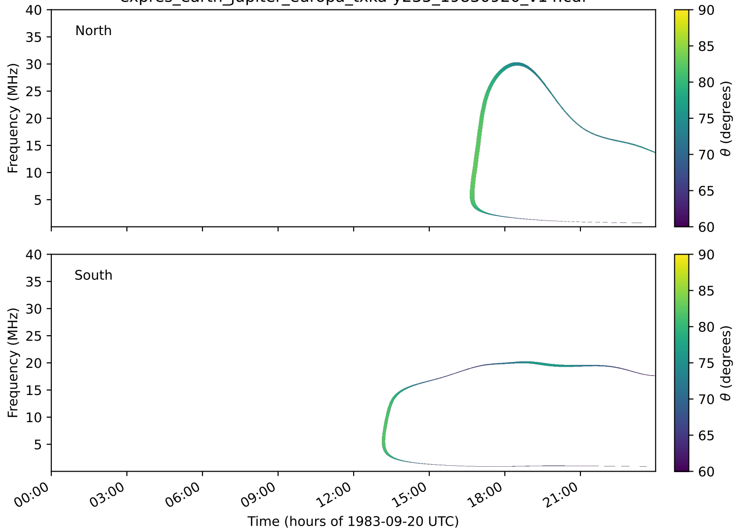
expres_earth_jupiter_europa_txka-y235_19830920_v14.cdf
