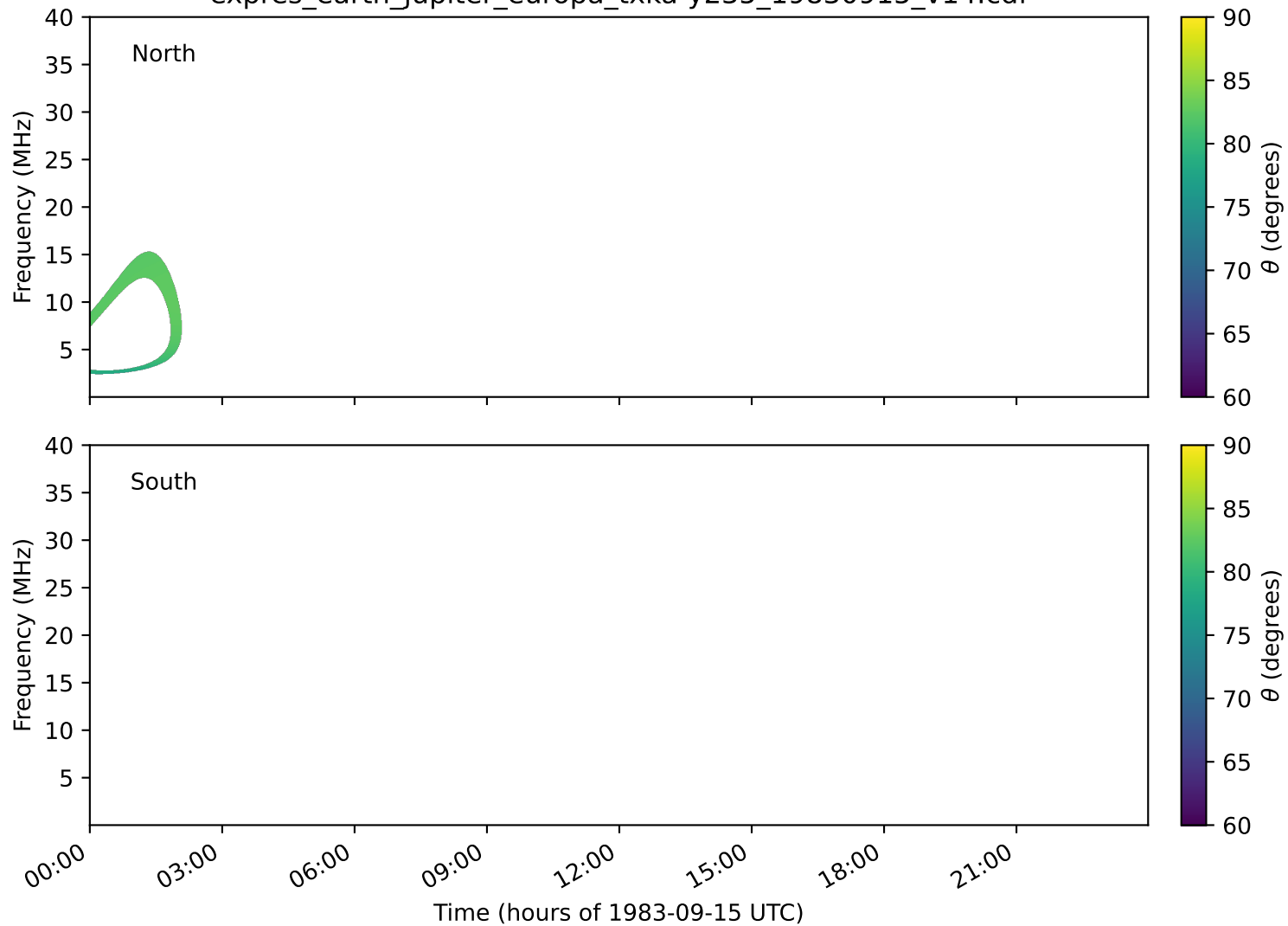
expres_earth_jupiter_europa_txka-y235_19830915_v14.cdf
