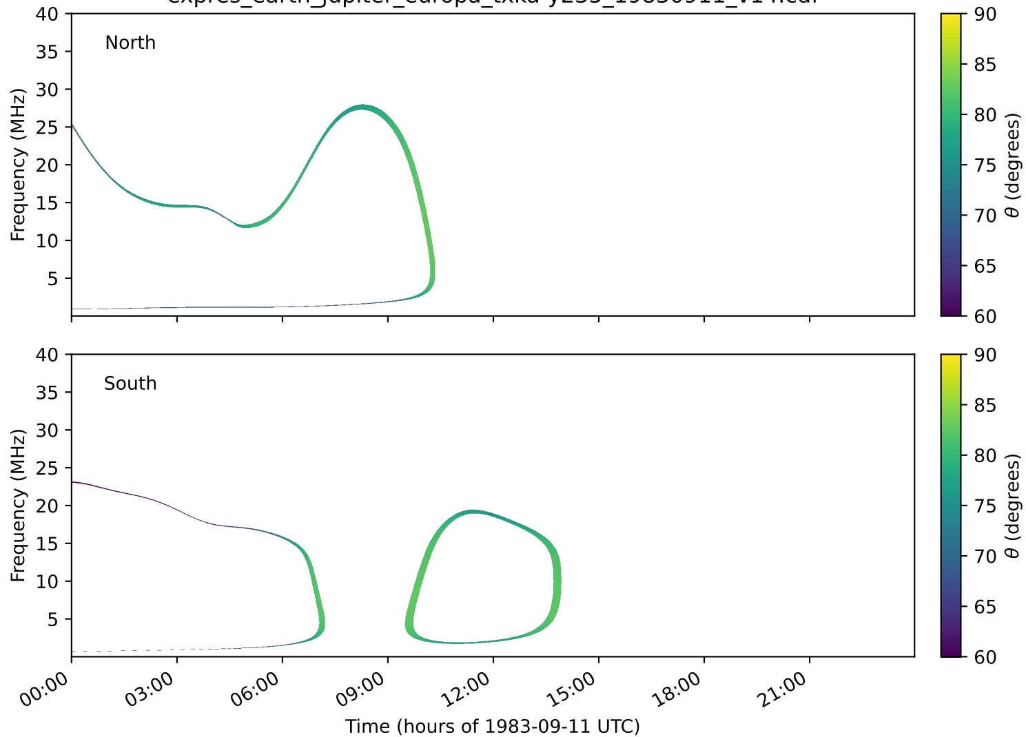
expres_earth_jupiter_europa_txka-y235_19830911_v14.cdf
