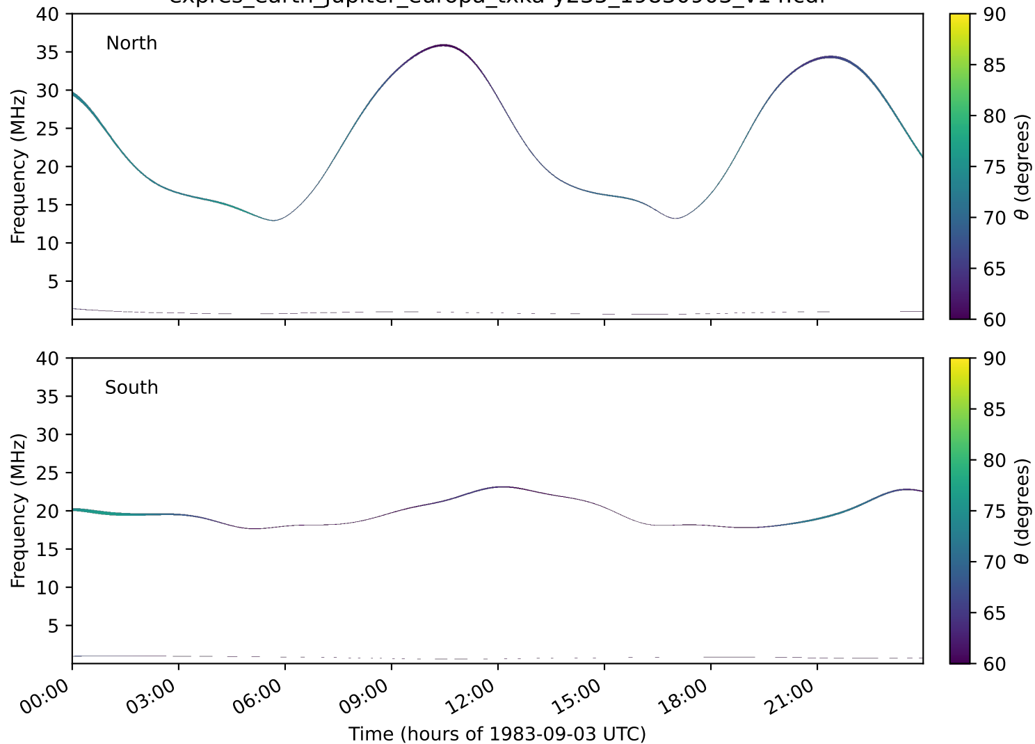
expres_earth_jupiter_europa_txka-y235_19830903_v14.cdf
