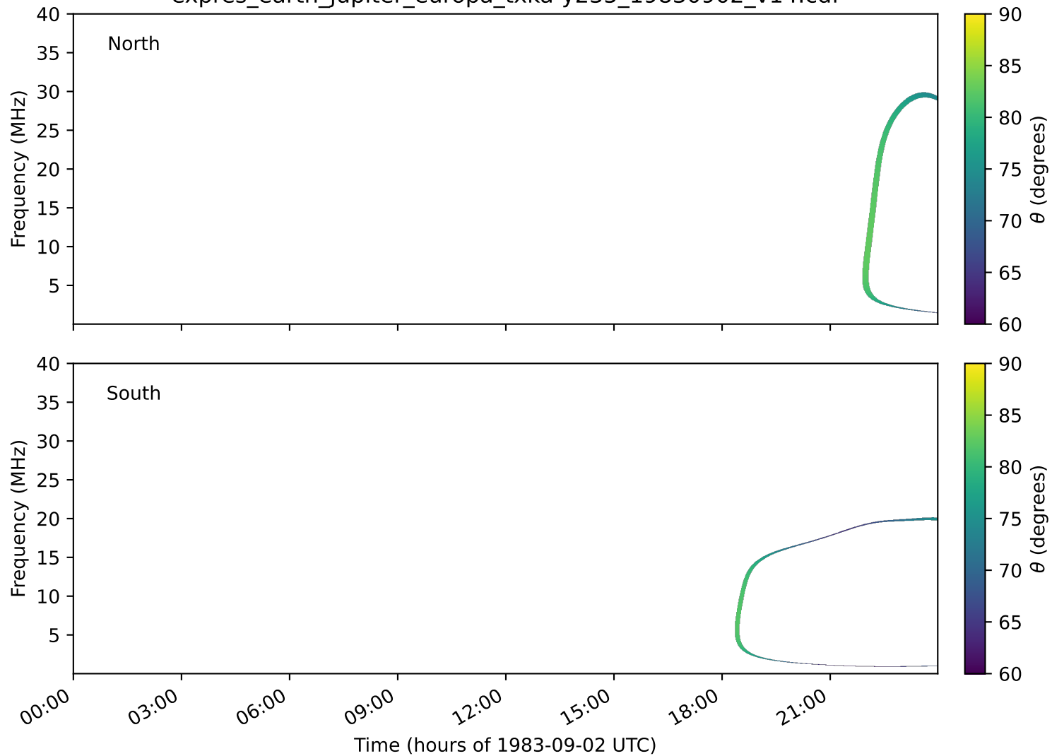
expres_earth_jupiter_europa_txka-y235_19830902_v14.cdf
