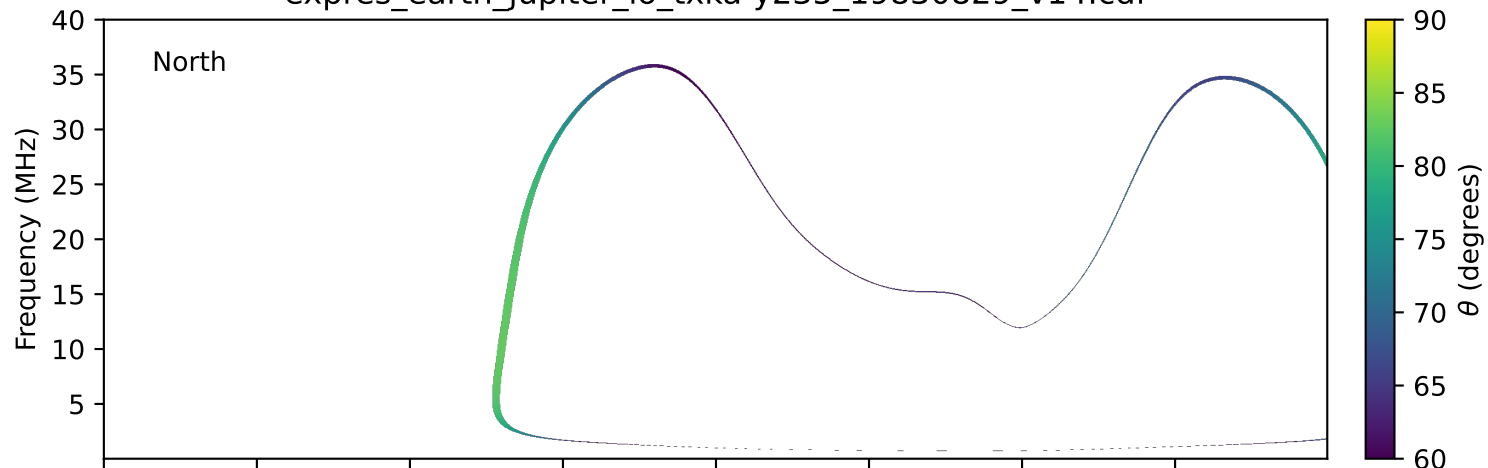
expres_earth_jupiter_io_txka-y235_19830829_v14.cdf
