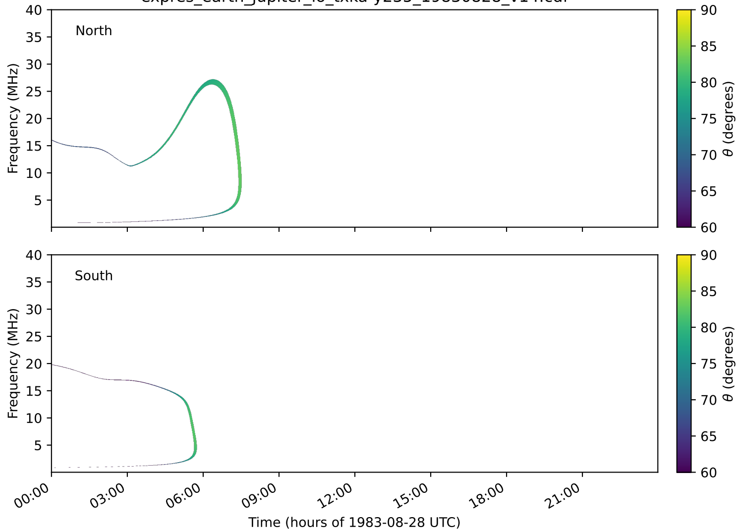
expres_earth_jupiter_io_txka-y235_19830828_v14.cdf
