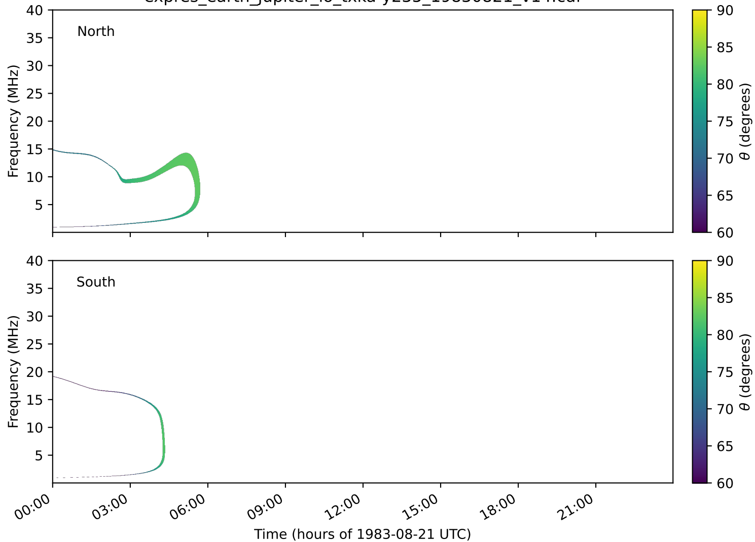
expres_earth_jupiter_io_txka-y235_19830821_v14.cdf
