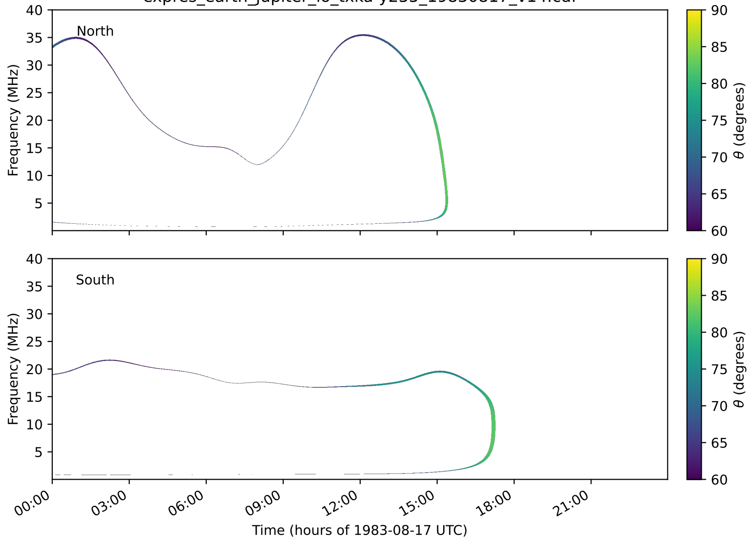
expres_earth_jupiter_io_txka-y235_19830817_v14.cdf
