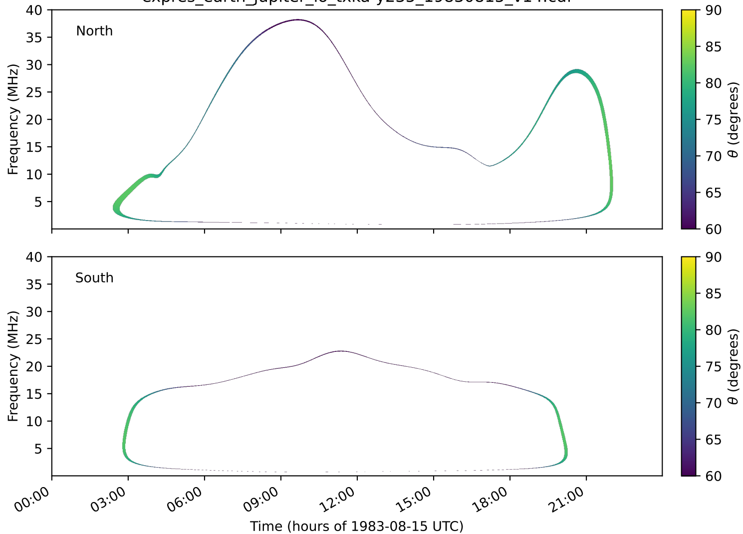
expres_earth_jupiter_io_txka-y235_19830815_v14.cdf
