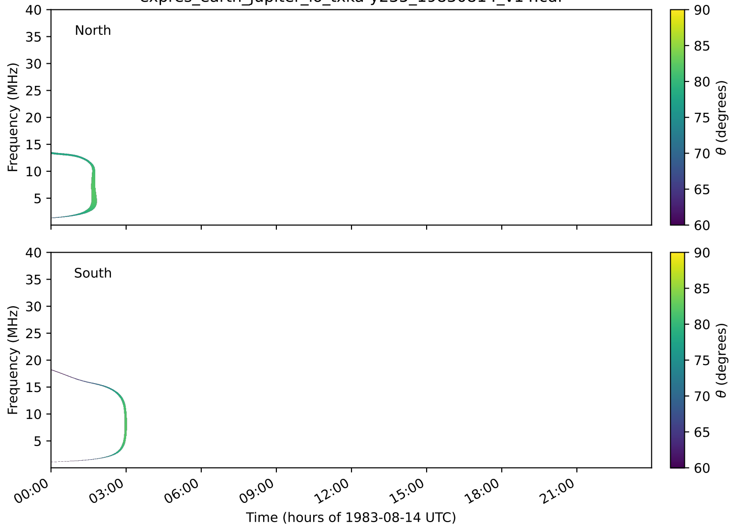
expres_earth_jupiter_io_txka-y235_19830814_v14.cdf
