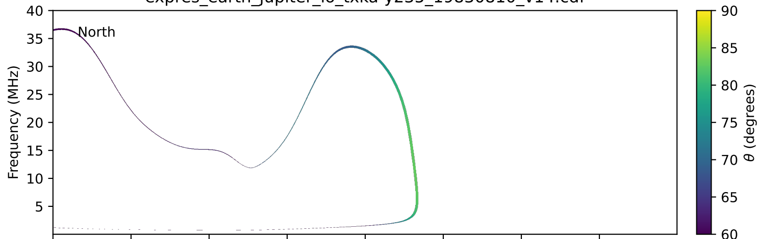
expres_earth_jupiter_io_txka-y235_19830810_v14.cdf
