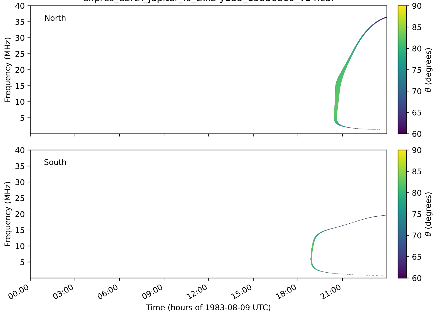
expres_earth_jupiter_io_txka-y235_19830809_v14.cdf
