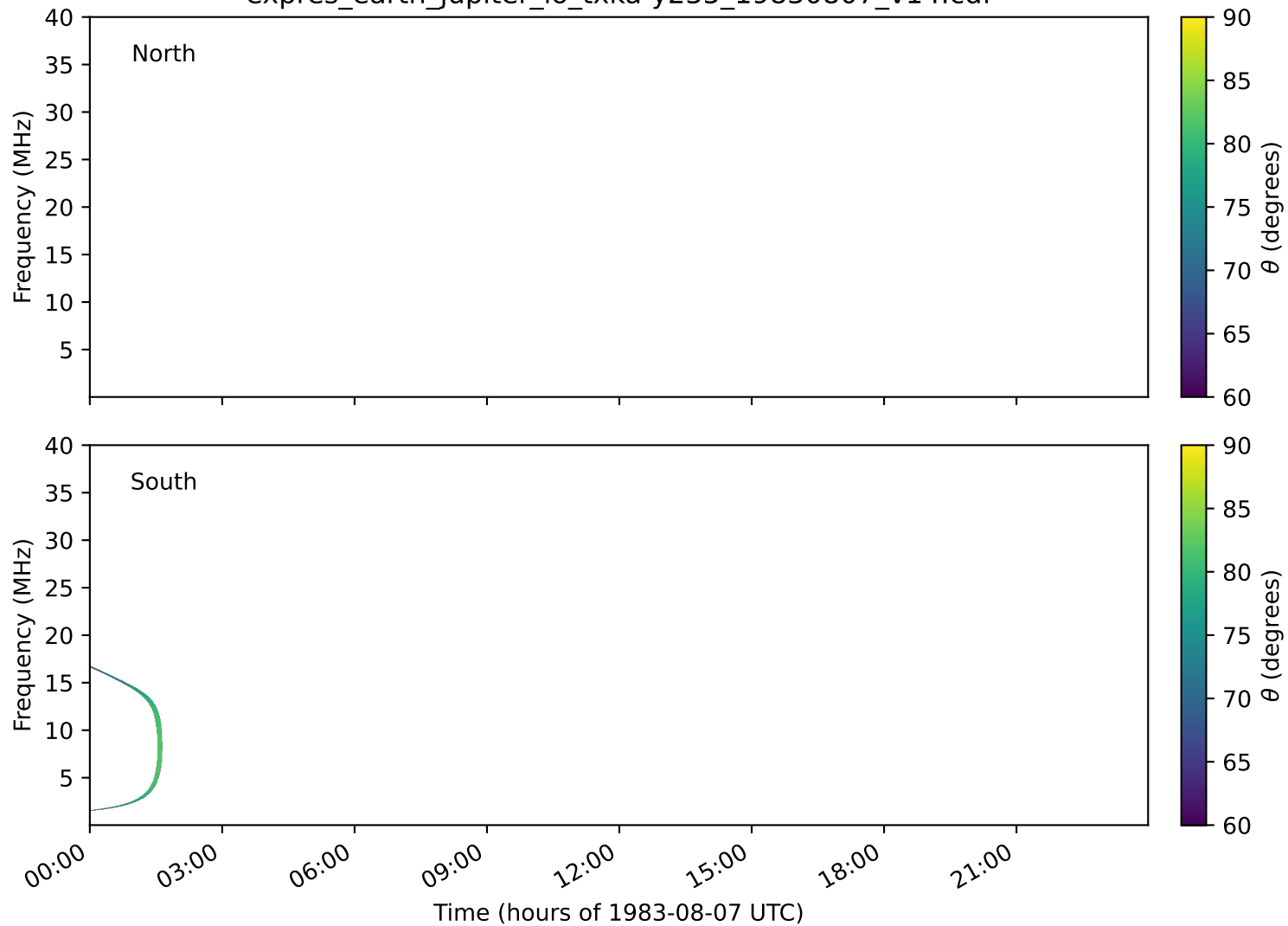
expres_earth_jupiter_io_txka-y235_19830807_v14.cdf
