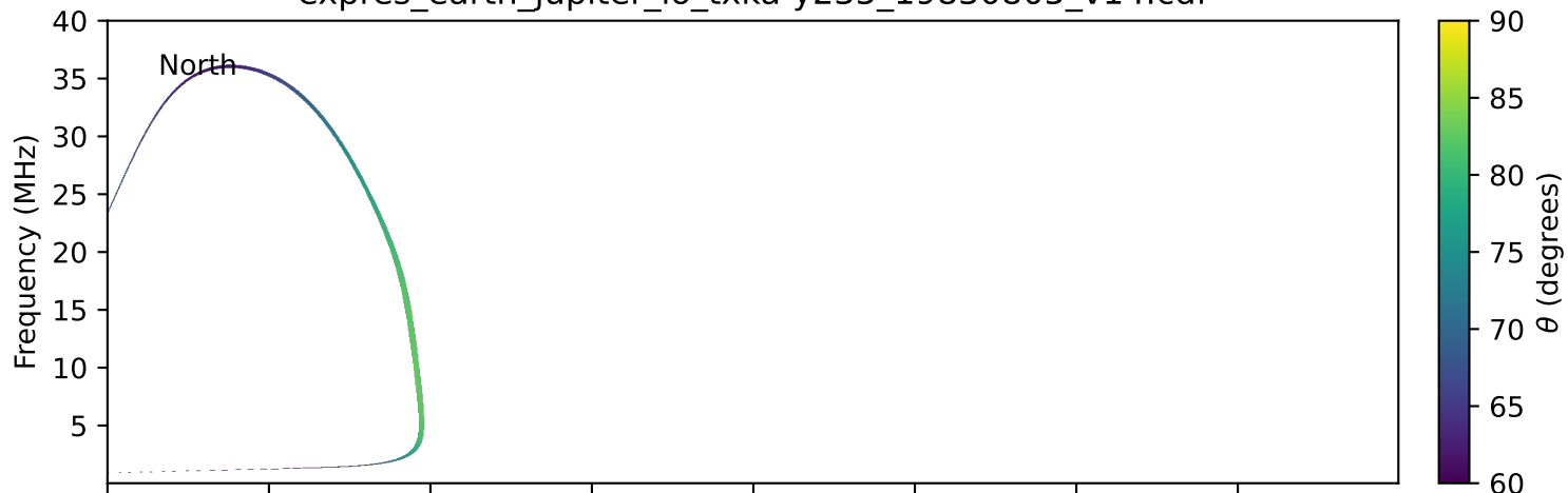
expres_earth_jupiter_io_txka-y235_19830805_v14.cdf
