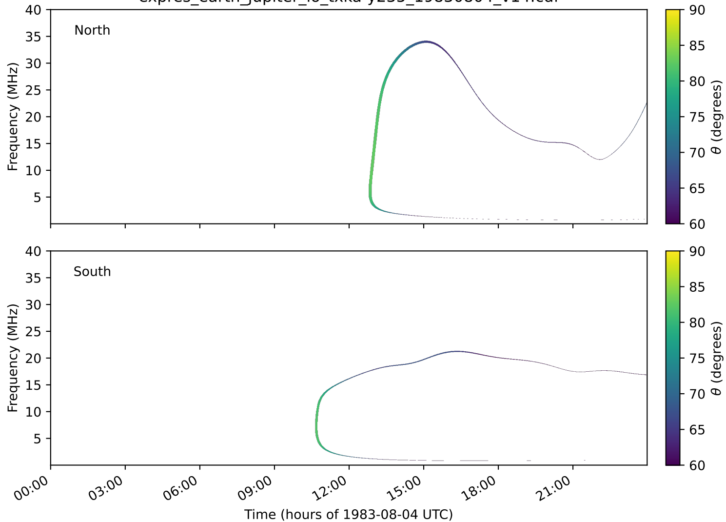
expres_earth_jupiter_io_txka-y235_19830804_v14.cdf
