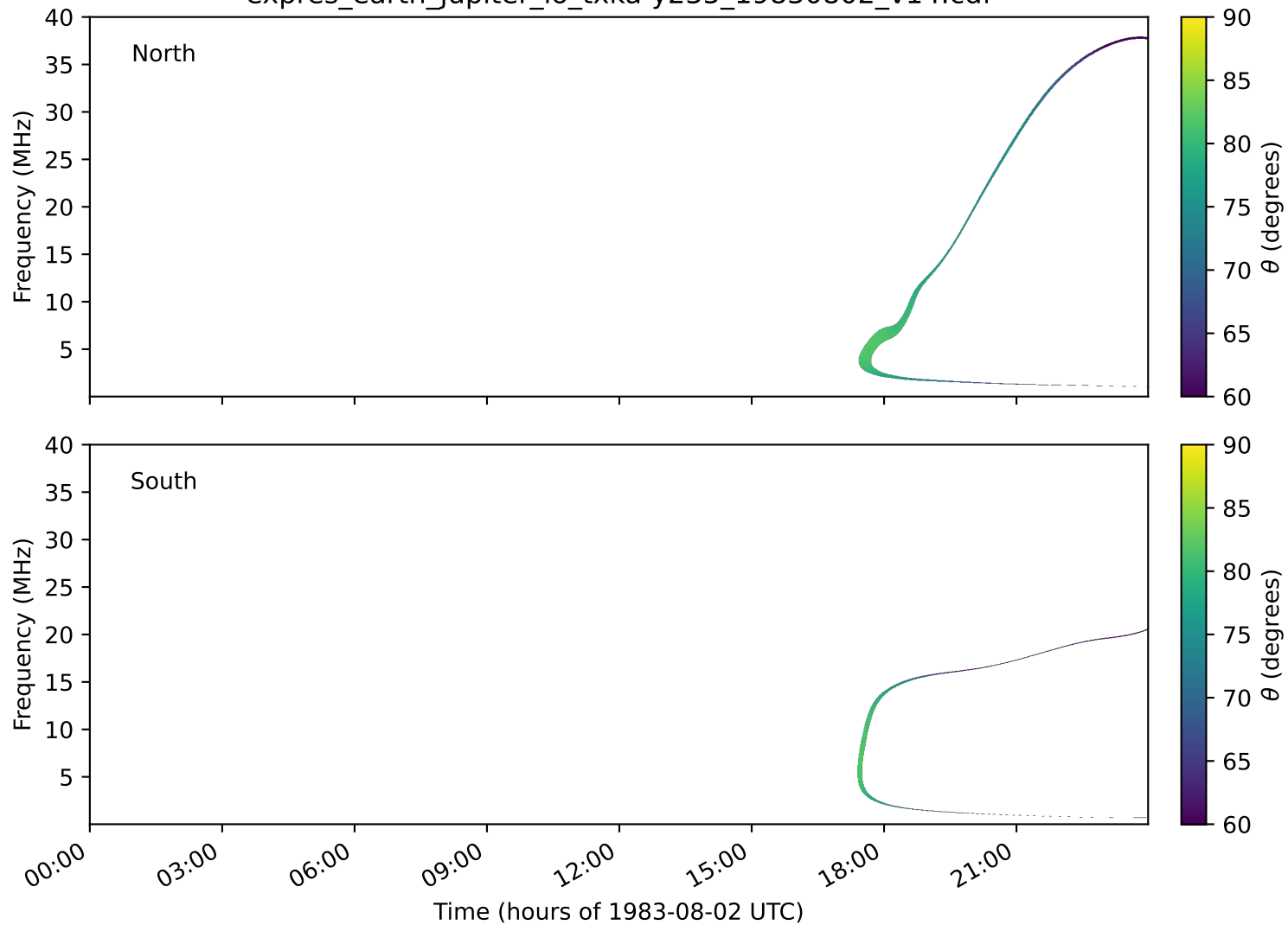
expres_earth_jupiter_io_txka-y235_19830802_v14.cdf
