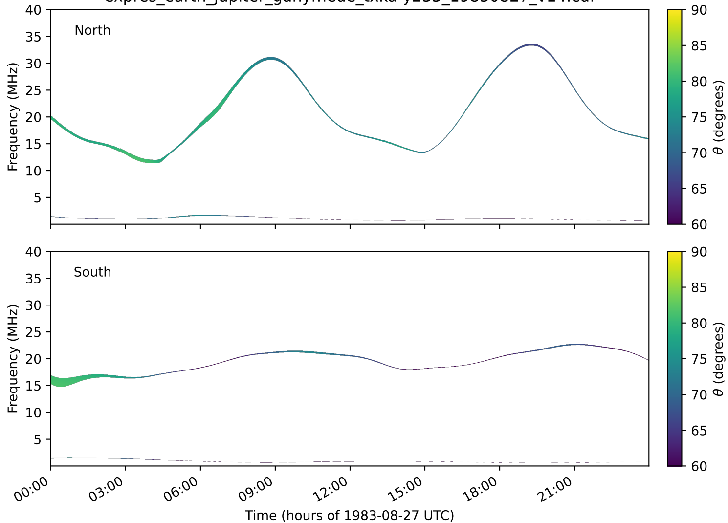
expres_earth_jupiter_ganymede_txka-y235_19830827_v14.cdf
