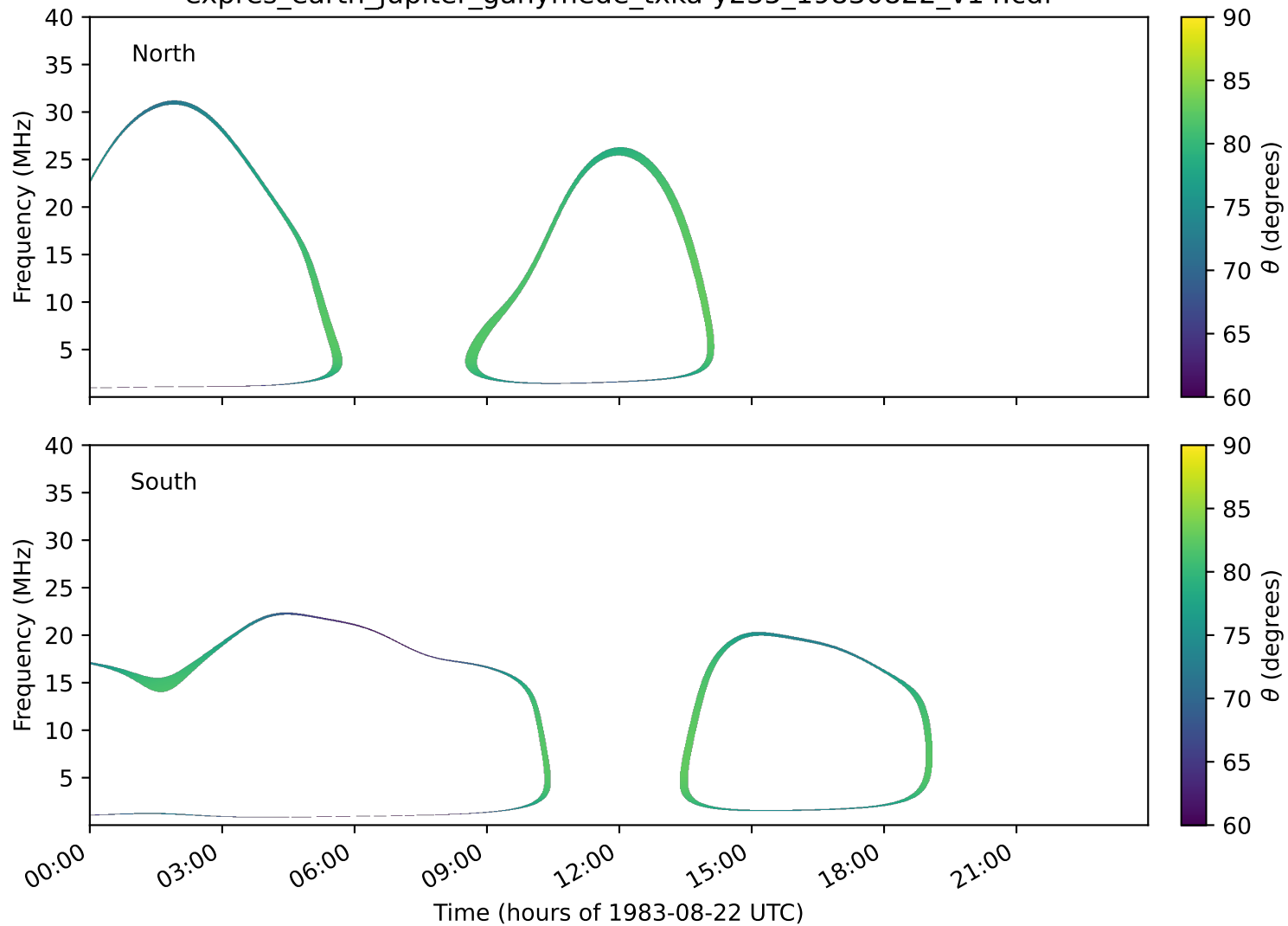
expres_earth_jupiter_ganymede_txka-y235_19830822_v14.cdf
