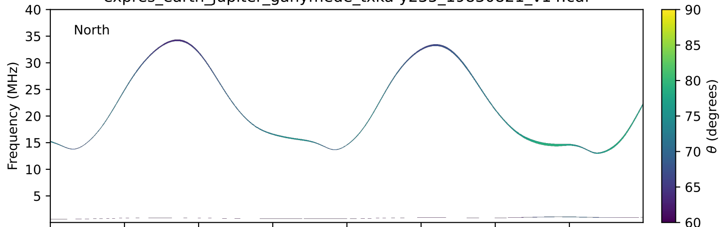
expres_earth_jupiter_ganymede_txka-y235_19830821_v14.cdf
