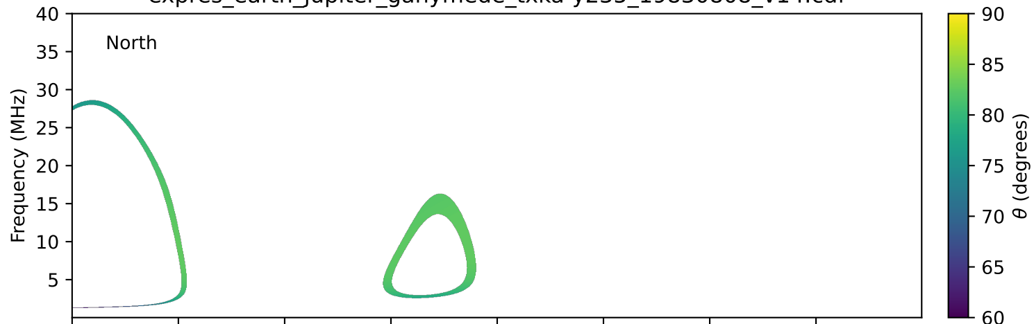
expres_earth_jupiter_ganymede_txka-y235_19830808_v14.cdf
