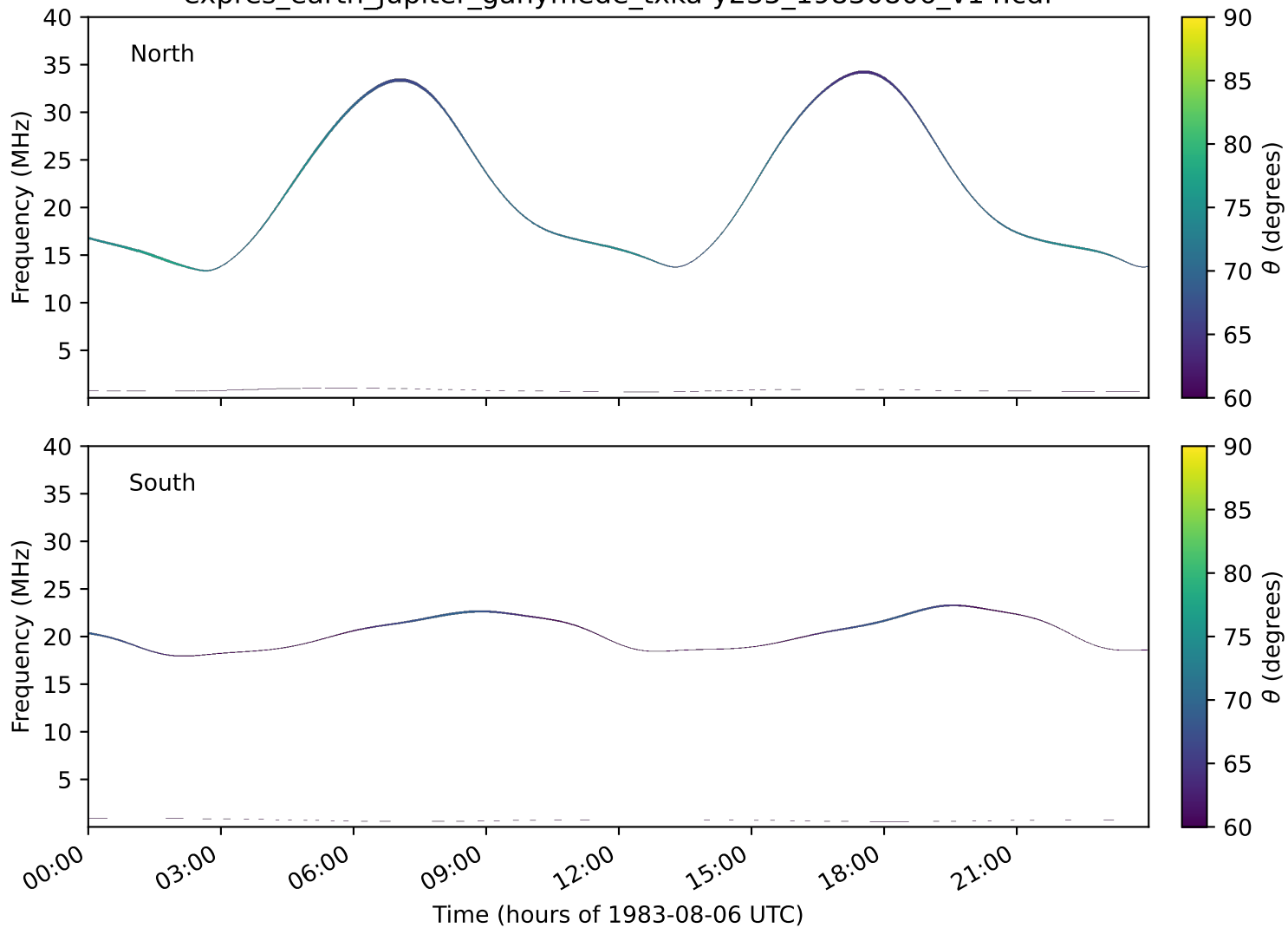
expres_earth_jupiter_ganymede_txka-y235_19830806_v14.cdf
