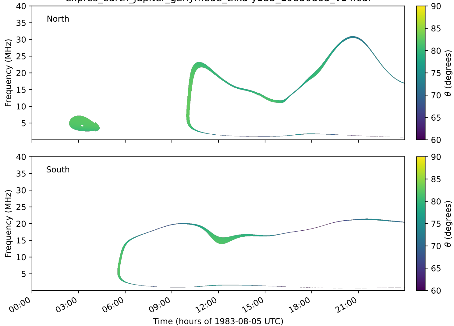
expres_earth_jupiter_ganymede_txka-y235_19830805_v14.cdf
