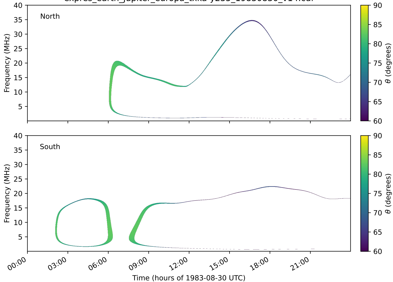
expres_earth_jupiter_europa_txka-y235_19830830_v14.cdf
