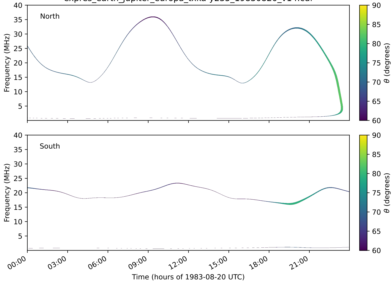
expres_earth_jupiter_europa_txka-y235_19830820_v14.cdf
