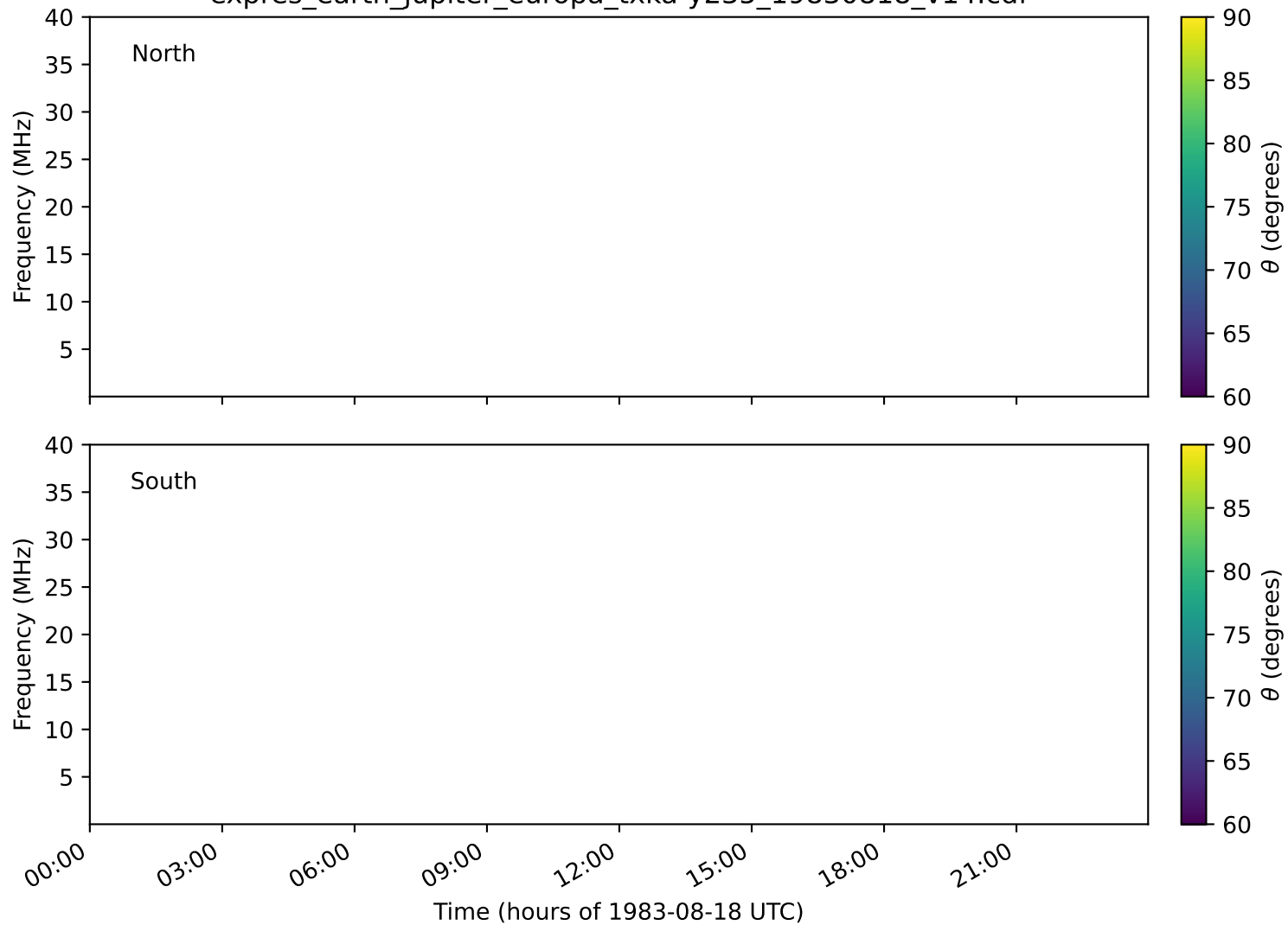
expres_earth_jupiter_europa_txka-y235_19830818_v14.cdf
