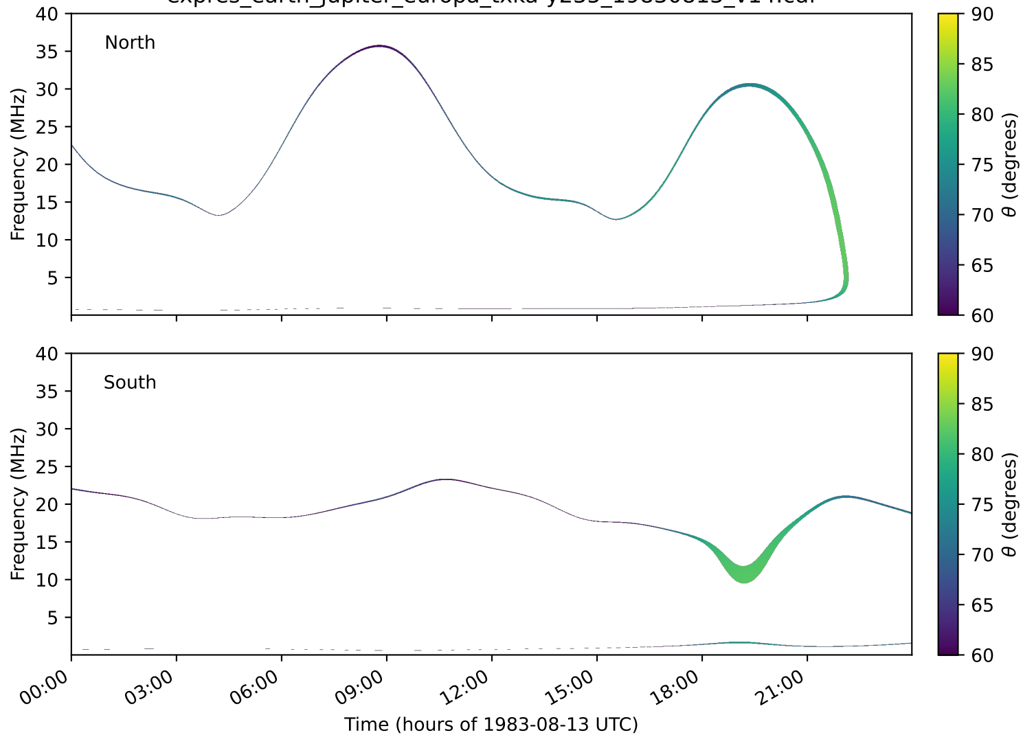
expres_earth_jupiter_europa_txka-y235_19830813_v14.cdf
