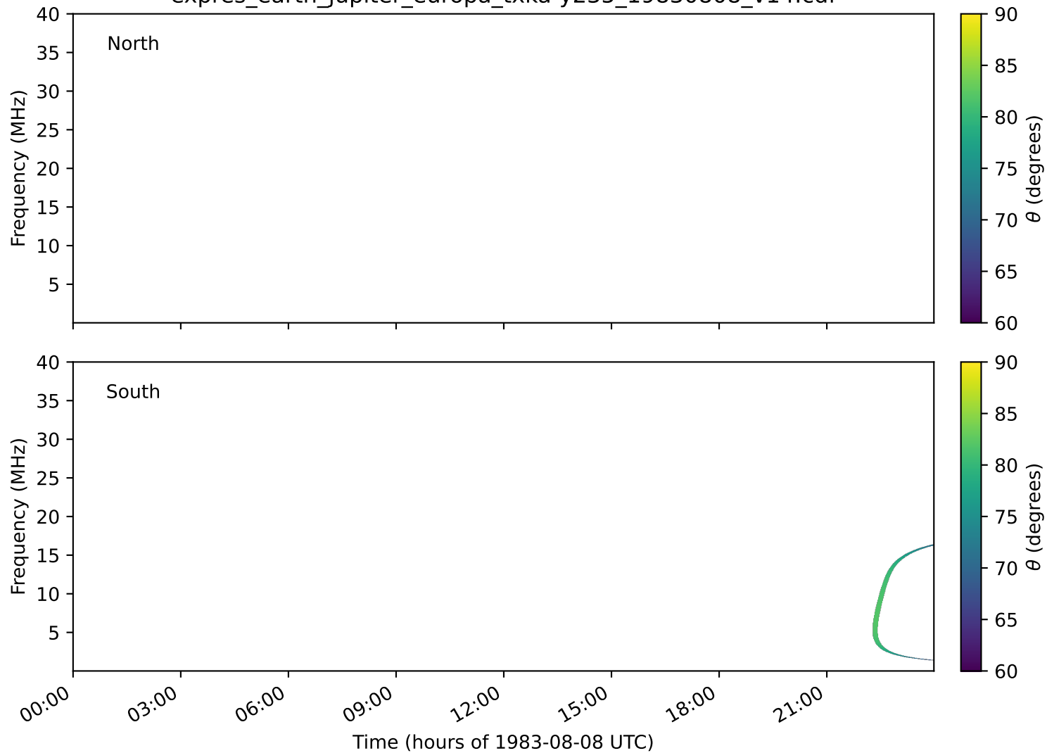
expres_earth_jupiter_europa_txka-y235_19830808_v14.cdf
