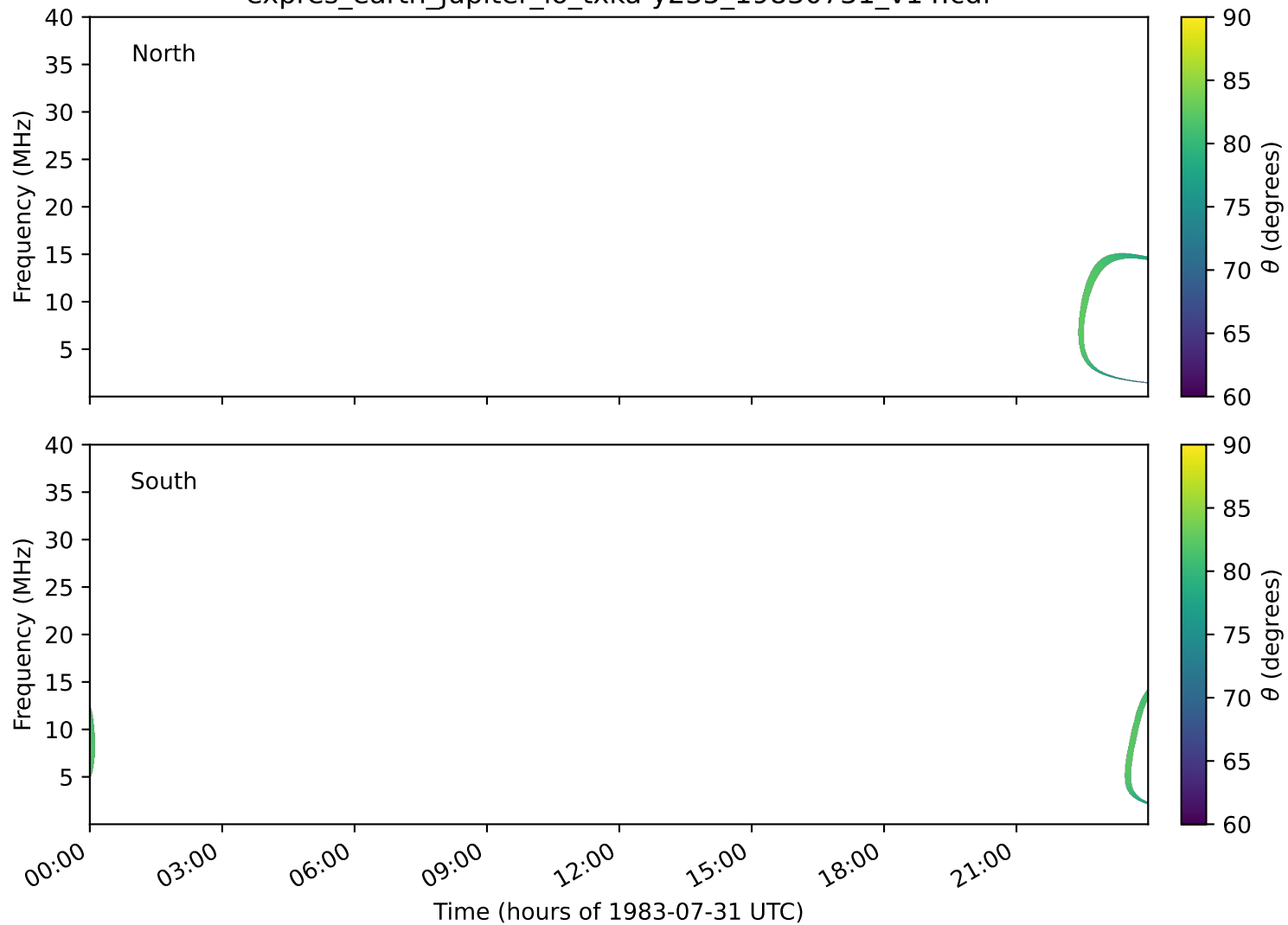
expres_earth_jupiter_io_txka-y235_19830731_v14.cdf
