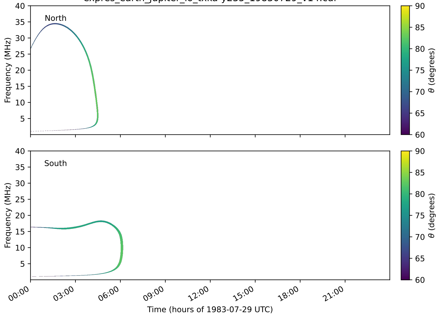
expres_earth_jupiter_io_txka-y235_19830729_v14.cdf
