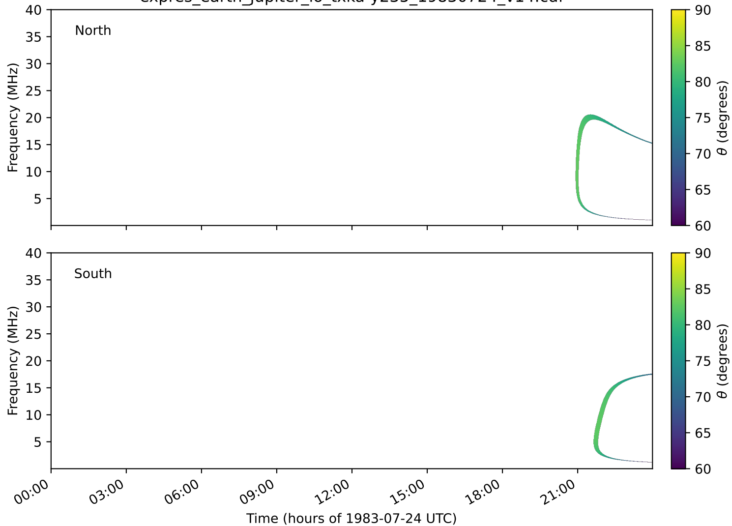
expres_earth_jupiter_io_txka-y235_19830724_v14.cdf
