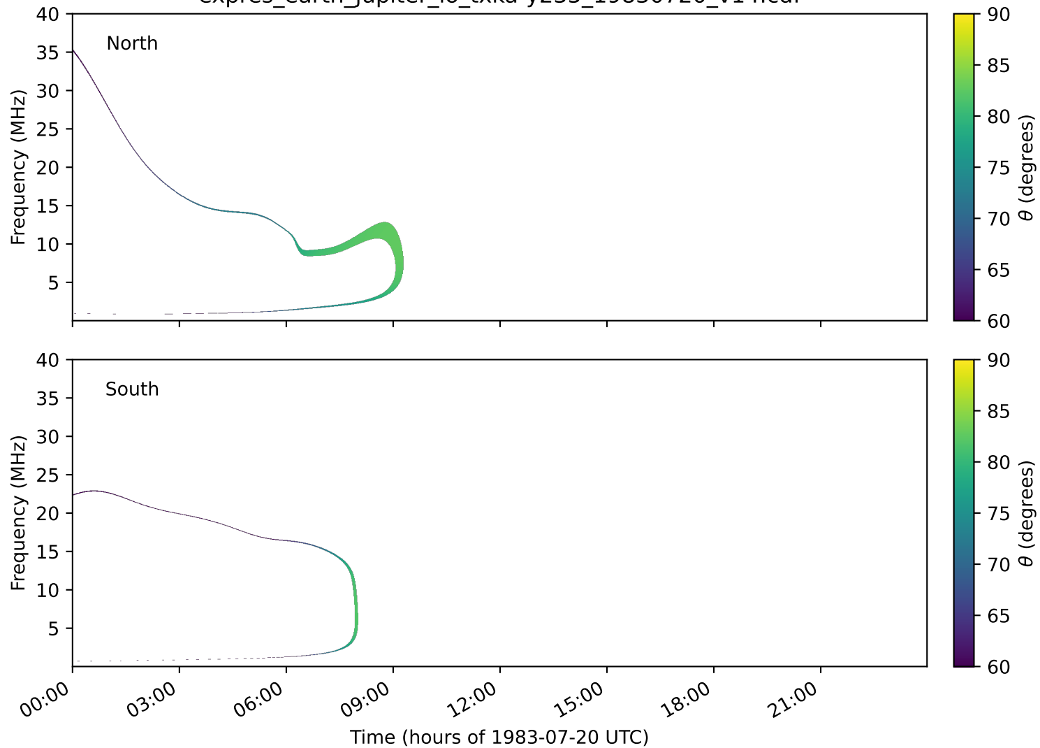
expres_earth_jupiter_io_txka-y235_19830720_v14.cdf
