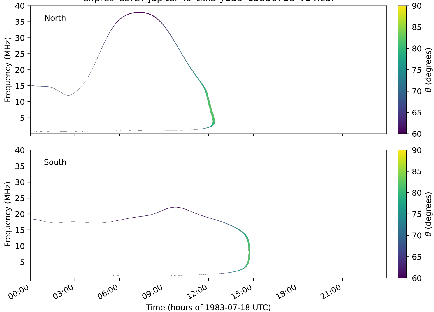
expres_earth_jupiter_io_txka-y235_19830718_v14.cdf
