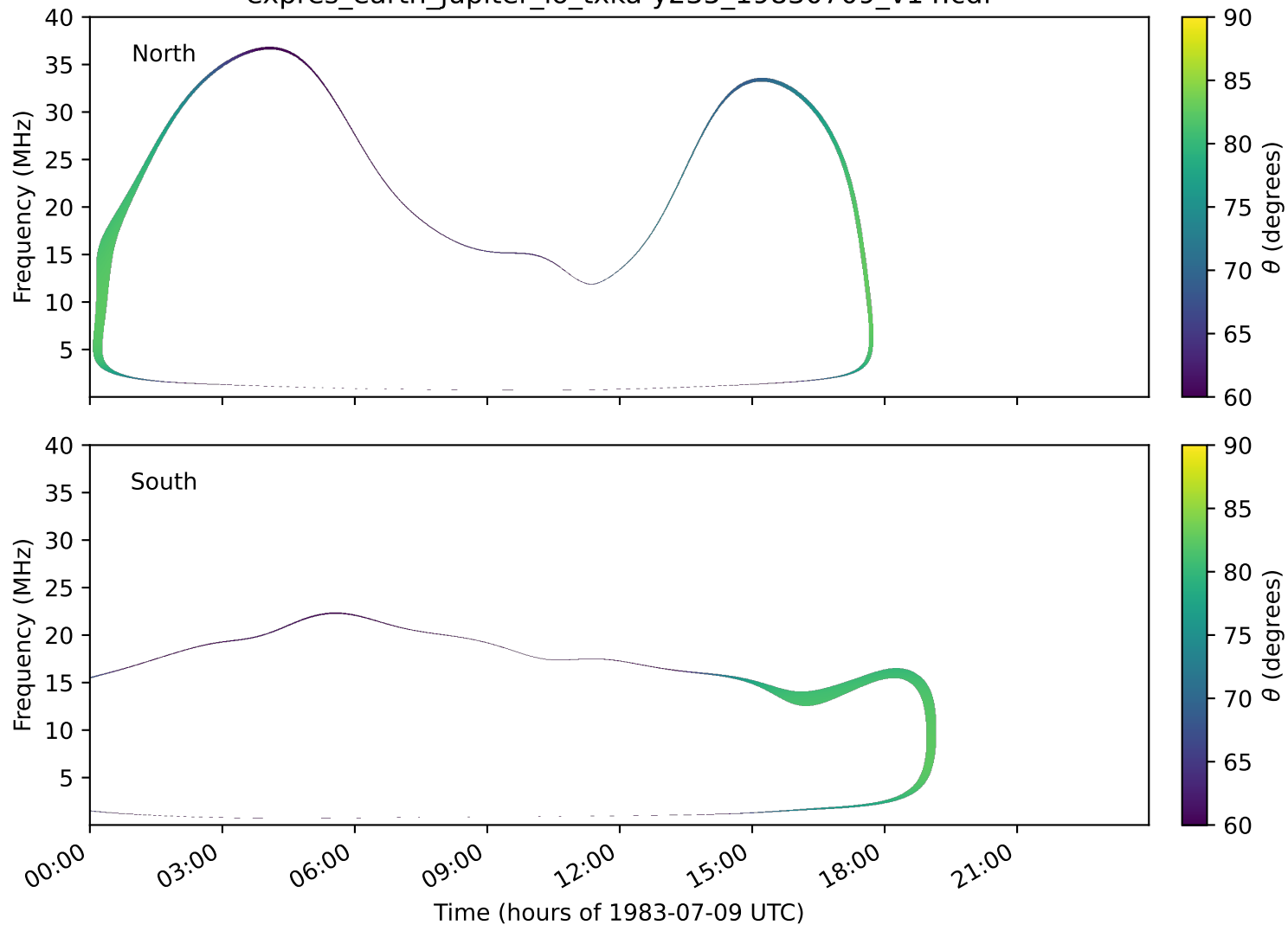
expres_earth_jupiter_io_txka-y235_19830709_v14.cdf
