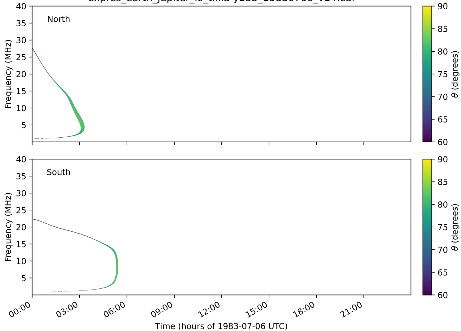
expres_earth_jupiter_io_txka-y235_19830706_v14.cdf
