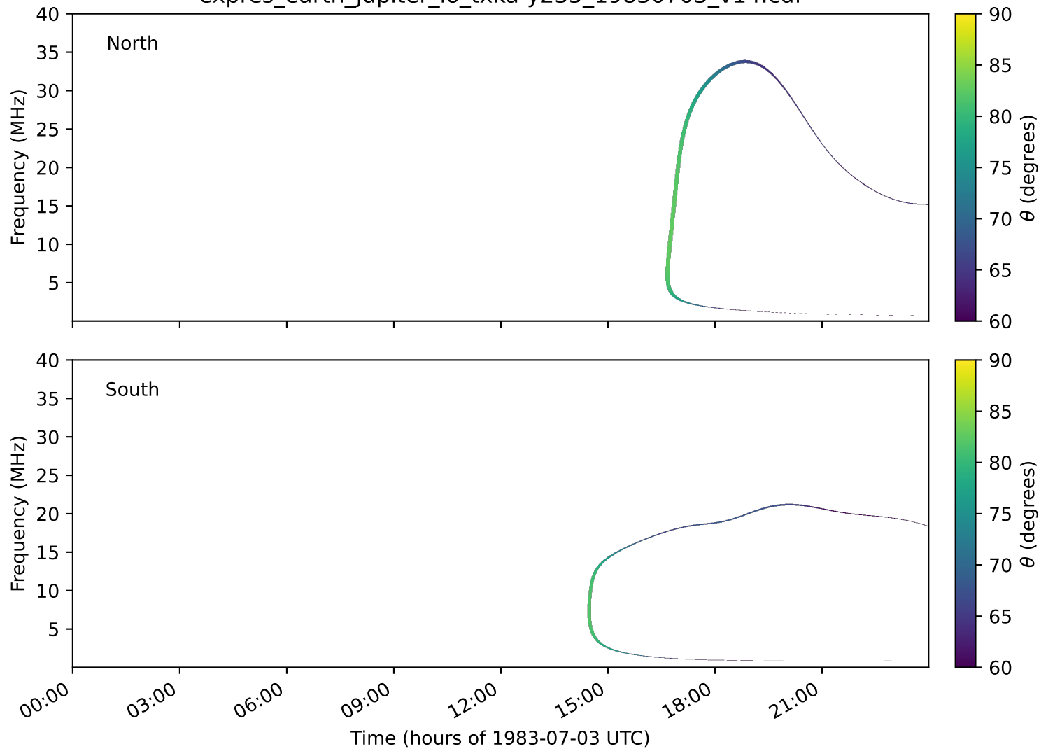
expres_earth_jupiter_io_txka-y235_19830703_v14.cdf
