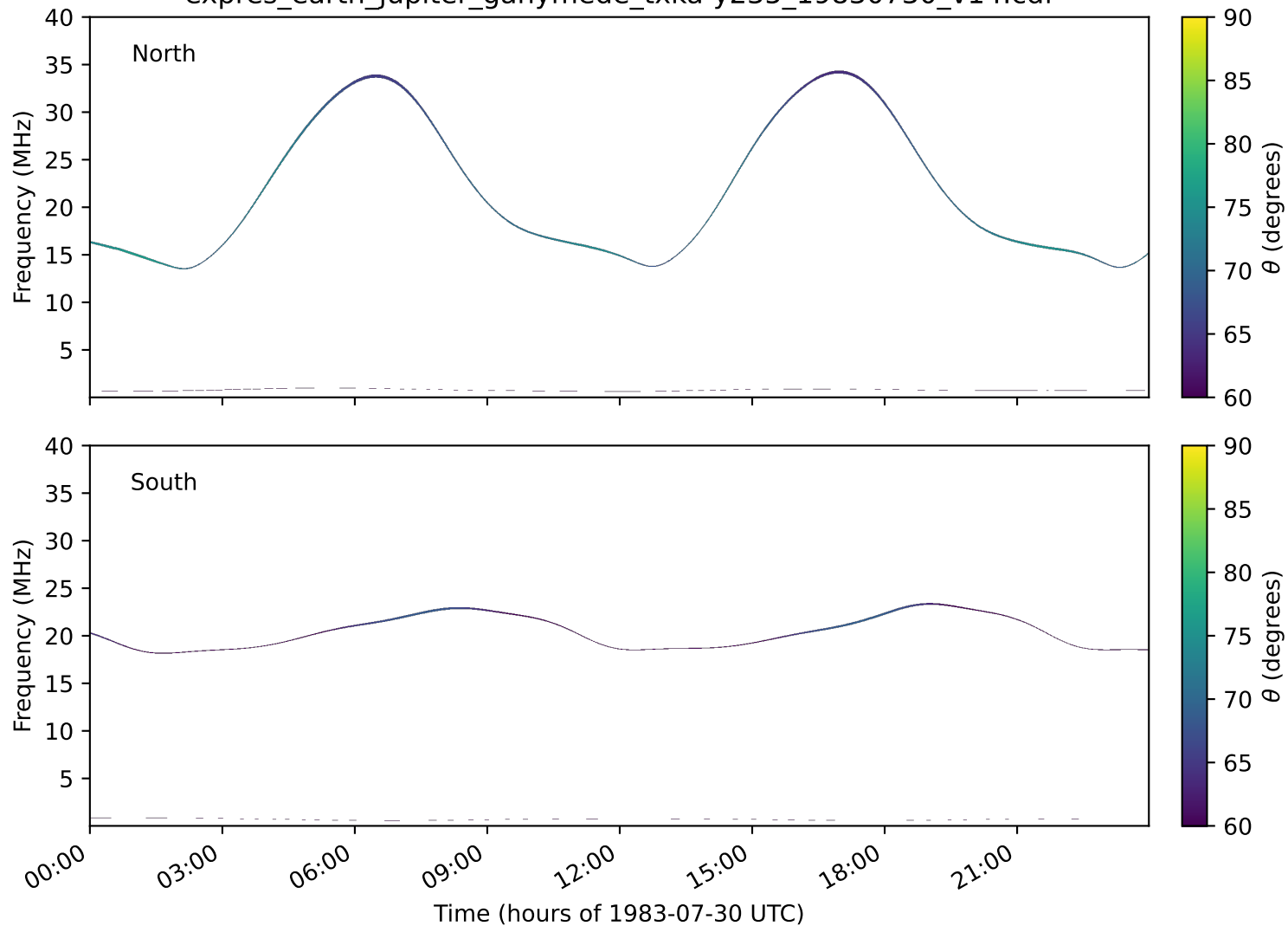
expres_earth_jupiter_ganymede_txka-y235_19830730_v14.cdf
