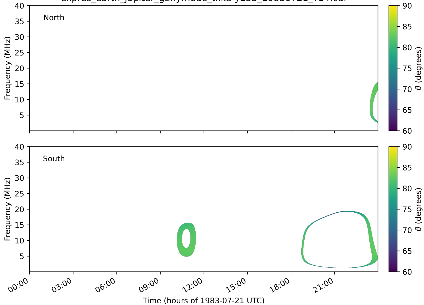
expres_earth_jupiter_ganymede_txka-y235_19830721_v14.cdf
