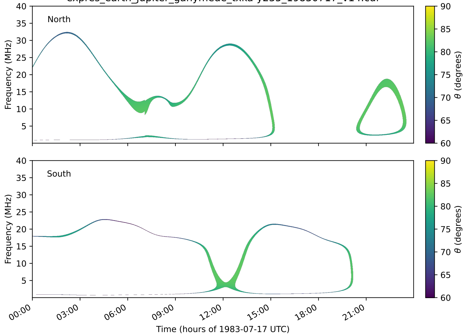
expres_earth_jupiter_ganymede_txka-y235_19830717_v14.cdf
