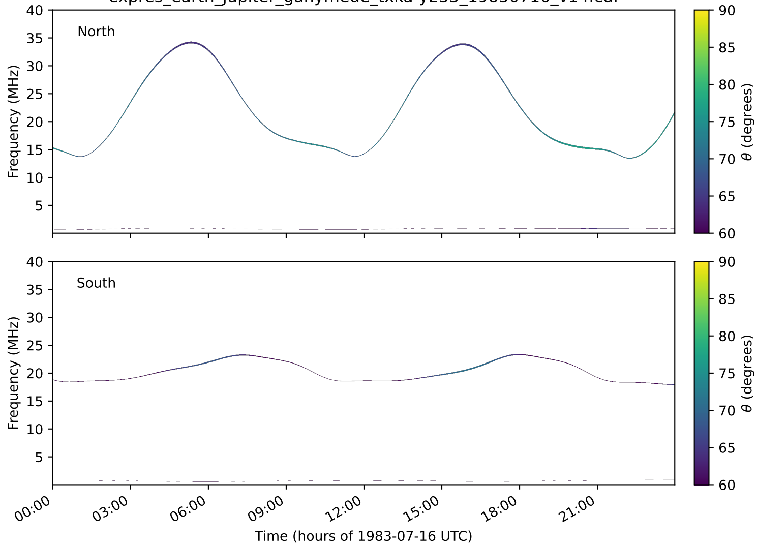
expres_earth_jupiter_ganymede_txka-y235_19830716_v14.cdf
