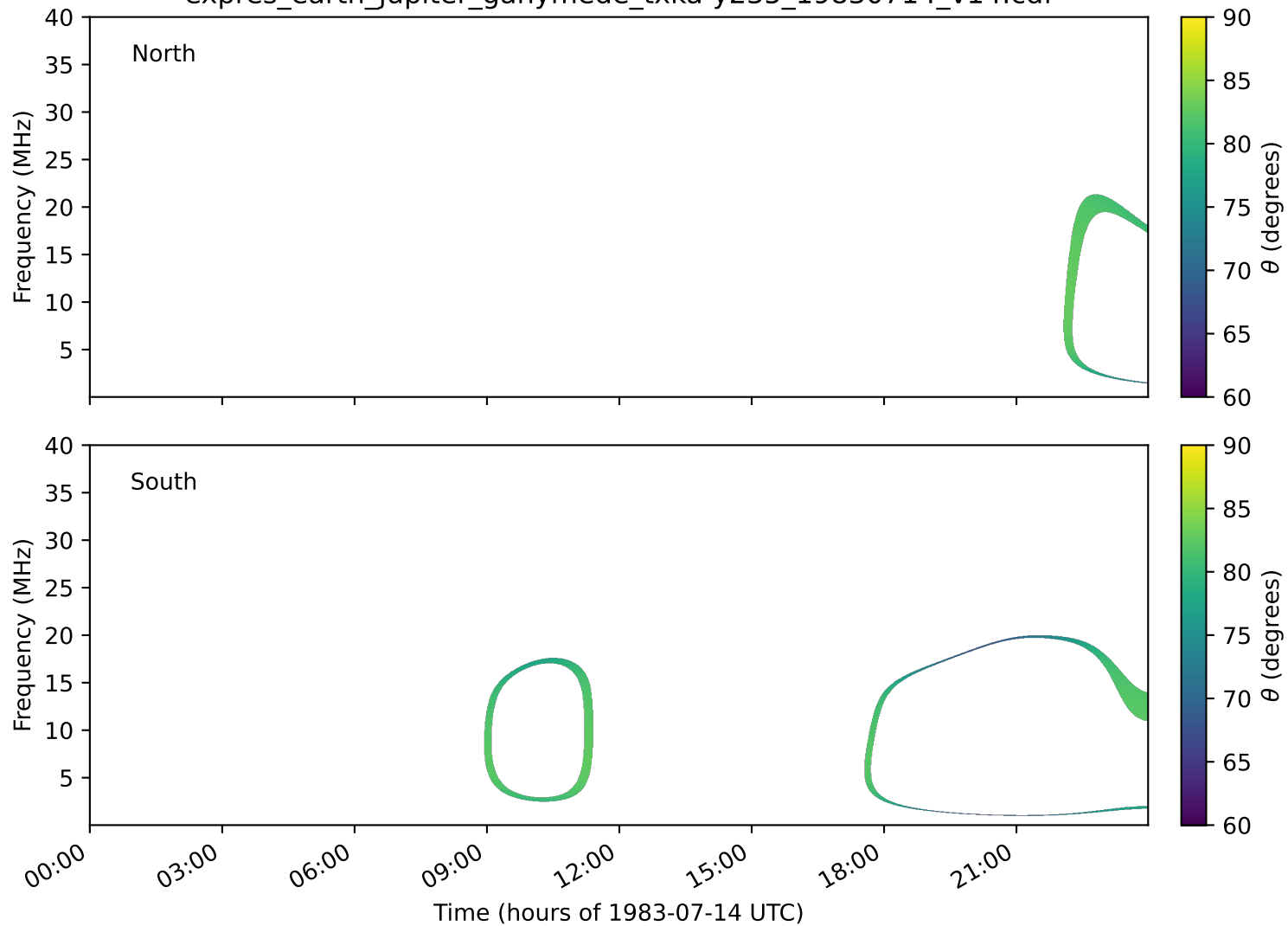
expres_earth_jupiter_ganymede_txka-y235_19830714_v14.cdf
