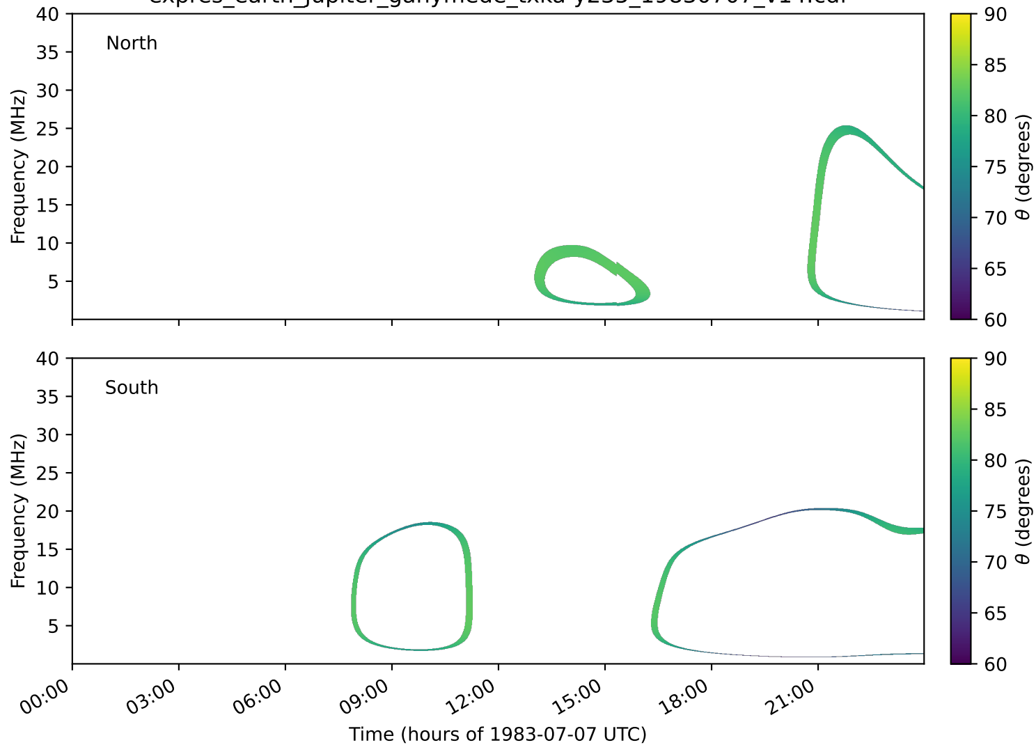
expres_earth_jupiter_ganymede_txka-y235_19830707_v14.cdf
