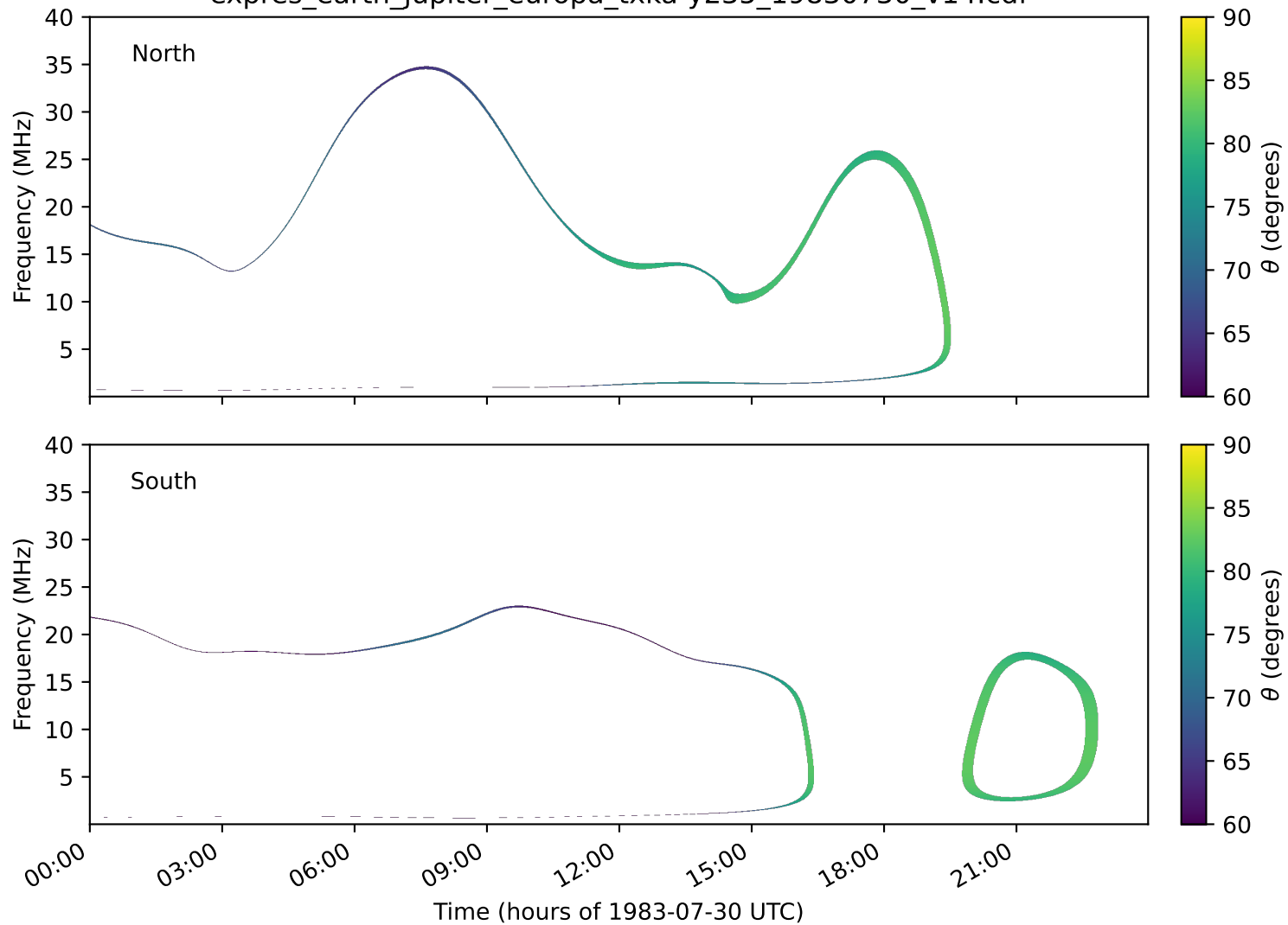
expres_earth_jupiter_europa_txka-y235_19830730_v14.cdf
