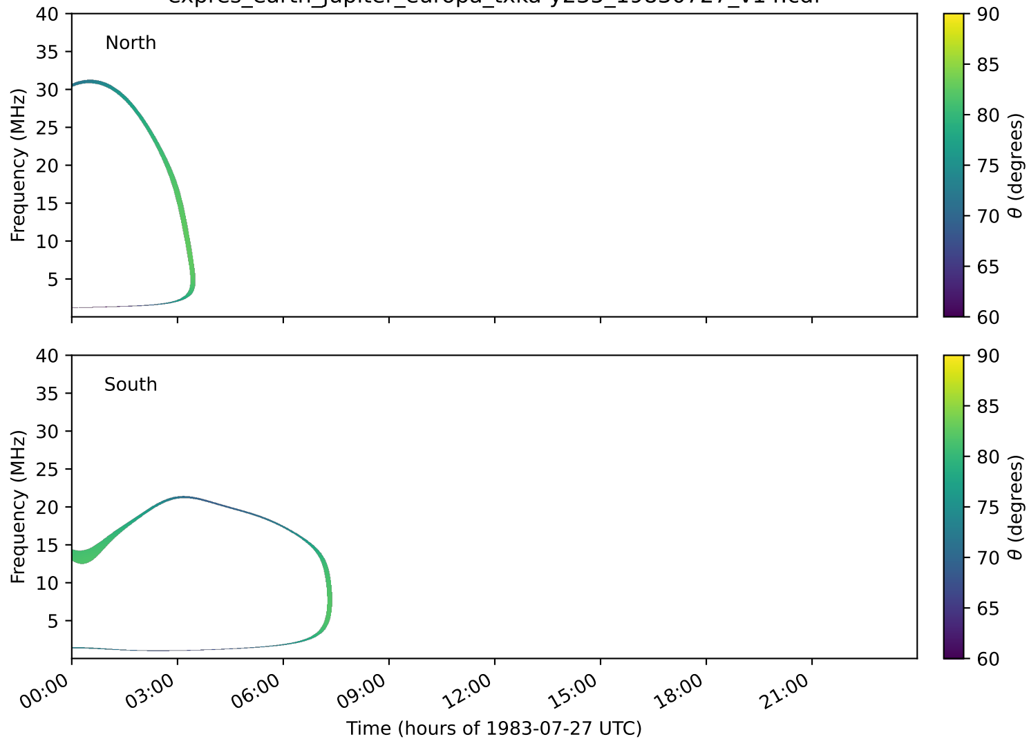
expres_earth_jupiter_europa_txka-y235_19830727_v14.cdf
