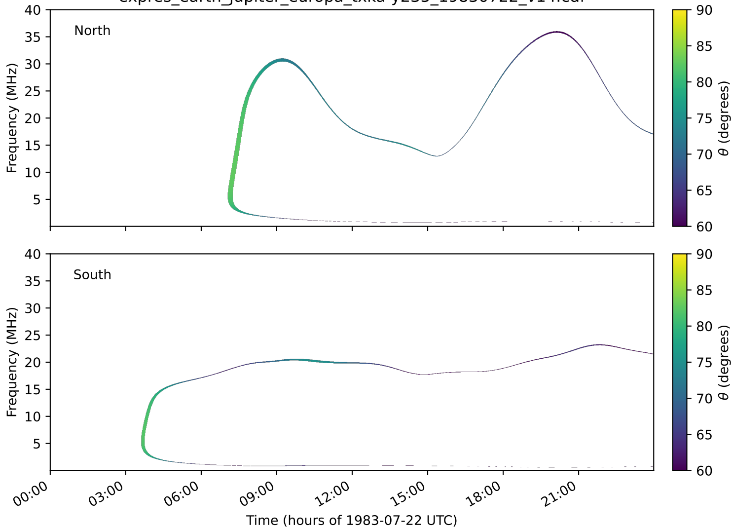
expres_earth_jupiter_europa_txka-y235_19830722_v14.cdf
