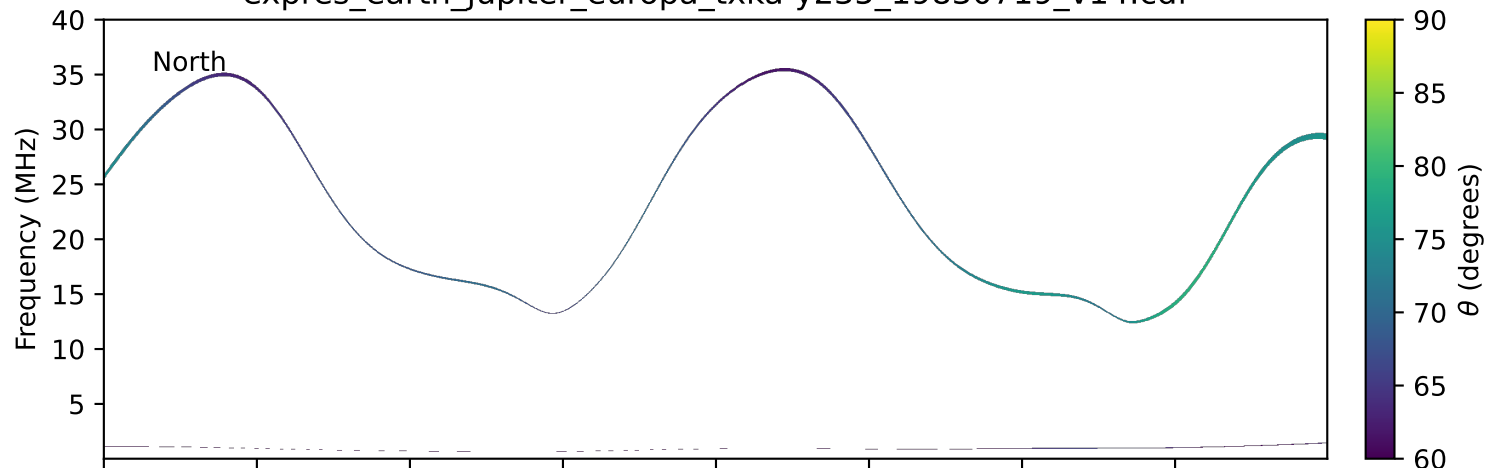
expres_earth_jupiter_europa_txka-y235_19830719_v14.cdf
